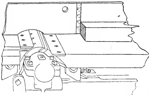
FIG. 145. DEPTH GAGE FOR JOINTER.
